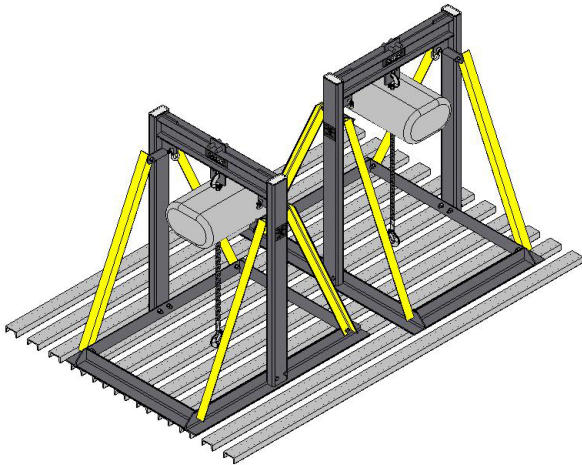
Chain Hoist on Grid
